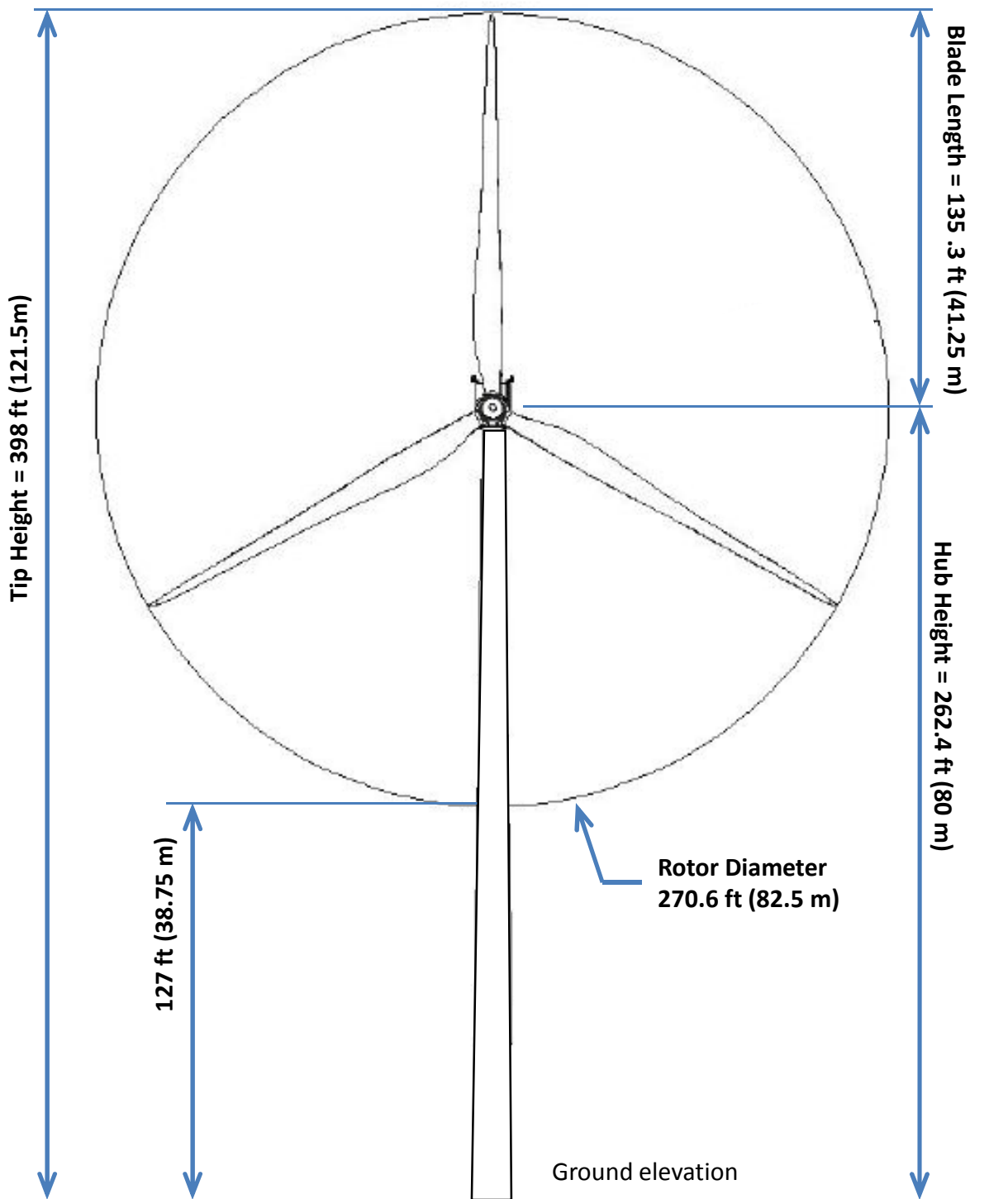
Figure 1. WTG Dimensions (Dimensions shown are for the GE 1.5xle and GE 1.6xle)
