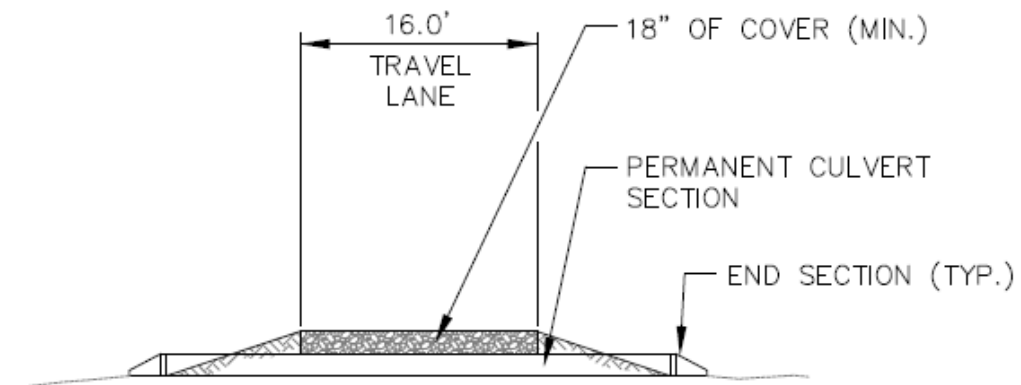
PERMANENT ACCESS ROADWAY CULVERT DETAIL – SECTION VIEW NOT TO SCALE
