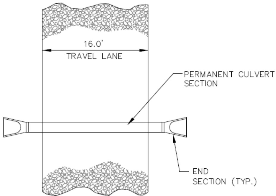
PERMANENT ACCESS ROADWAY CULVERT DETAIL – PLAN VIEW NOT TO SCALE
