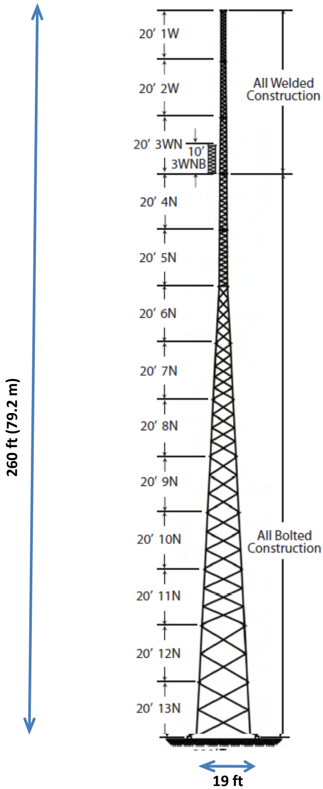
Figure 7. Permanent Met Tower
