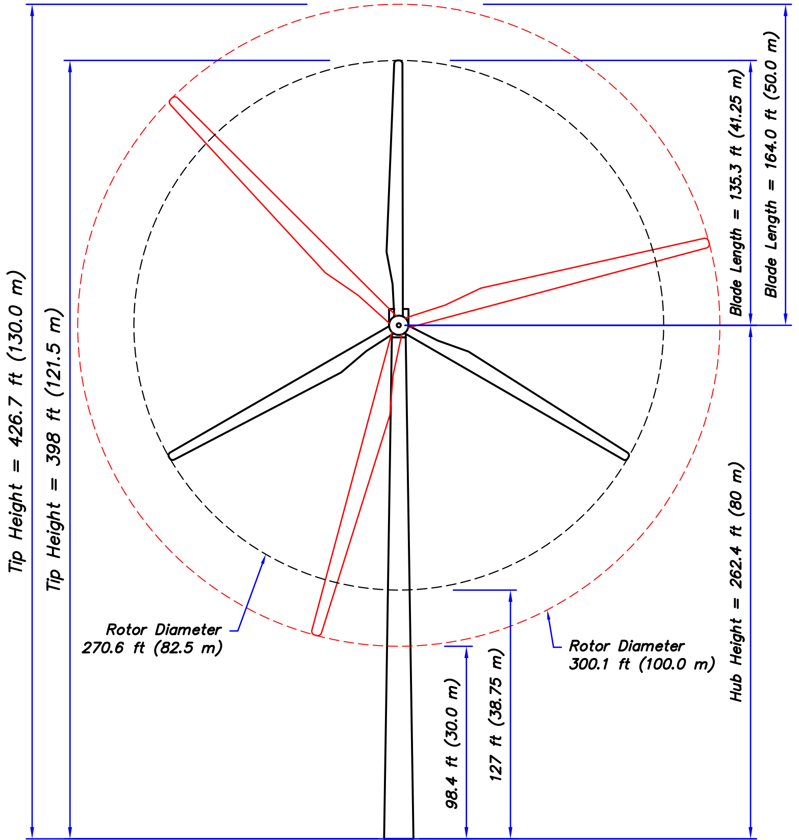
Figure 1. WTG Dimensions (Dimensions shown are for the GE 1.5xle and GE 1.6xle)
