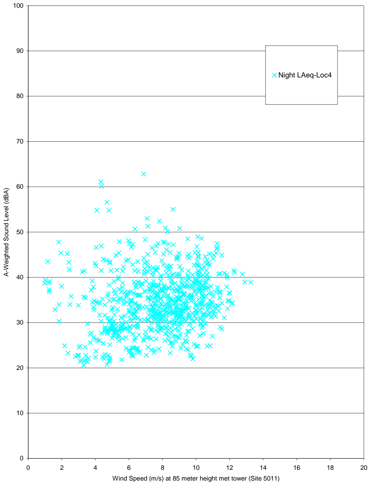
Figure 15h. Nighttime A-Weighted Leq Sound Levels vs. Wind Speed Measured at 10-Minute Intervals at Location 4 (23 July – 7 August 2009).
