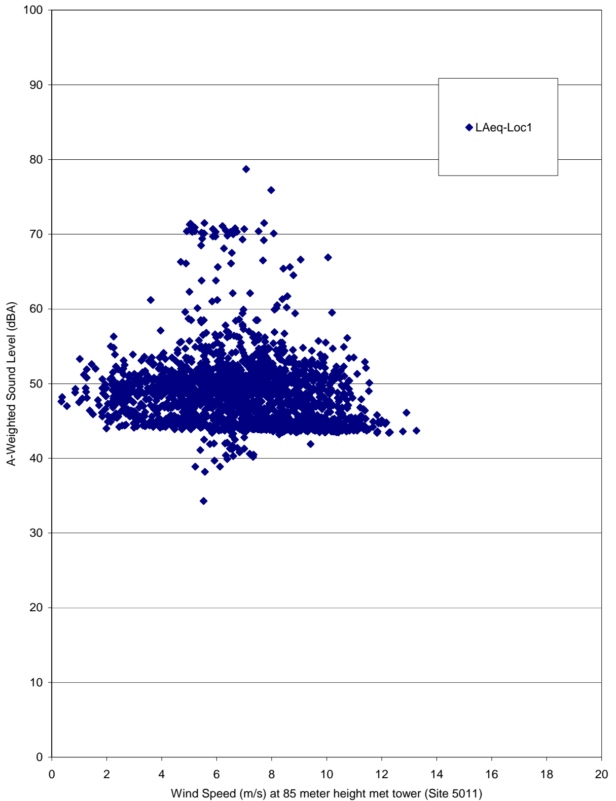
Figure 15a. A-Weighted Leq Sound Levels vs. Wind Speed Measured at 10-Minute Intervals at Location 1 (23 July – 7 August 2009).
