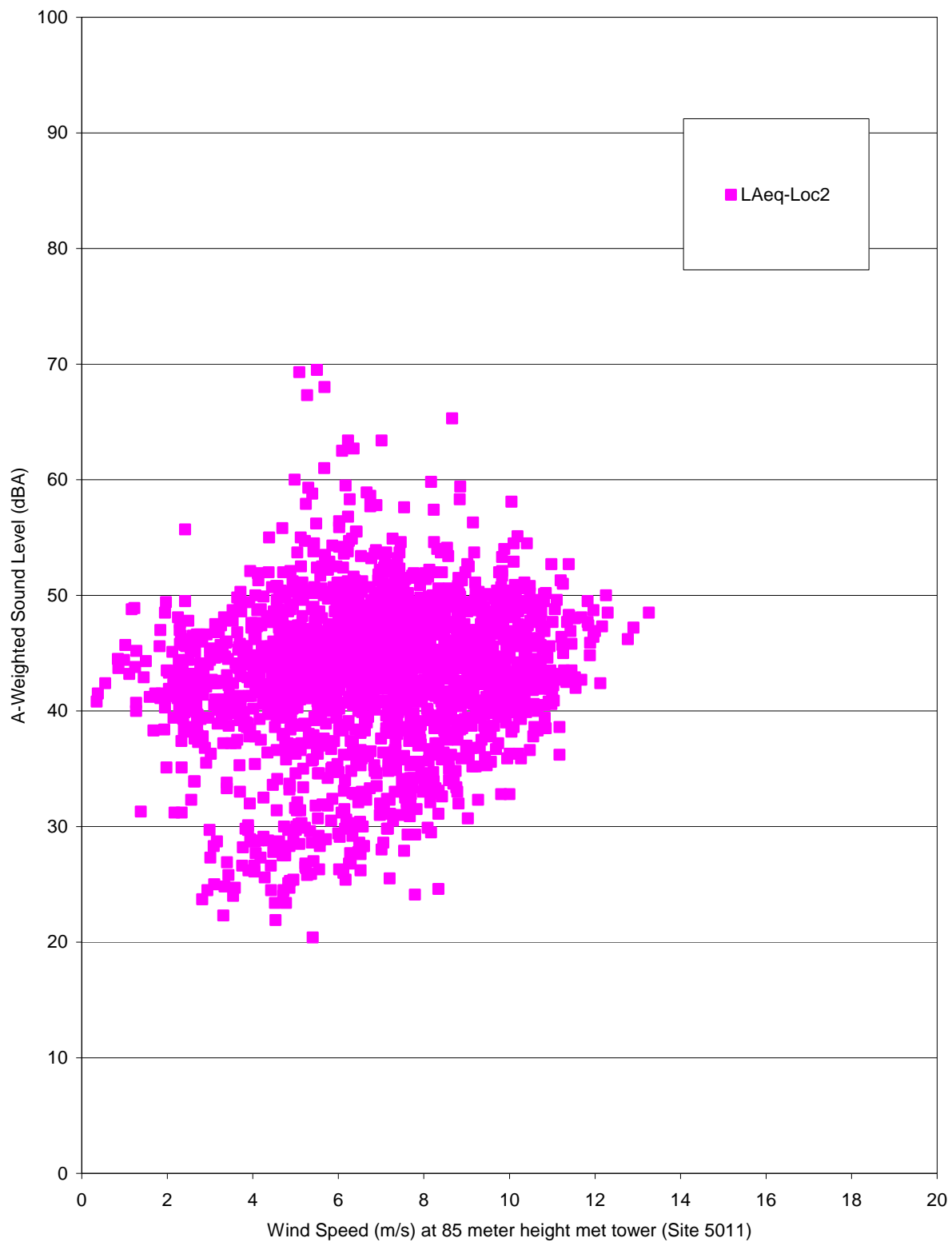
Figure 15b. A-Weighted Leq Sound Levels vs. Wind Speed Measured at 10-Minute Intervals at Location 2 (23 July – 7 August 2009).
