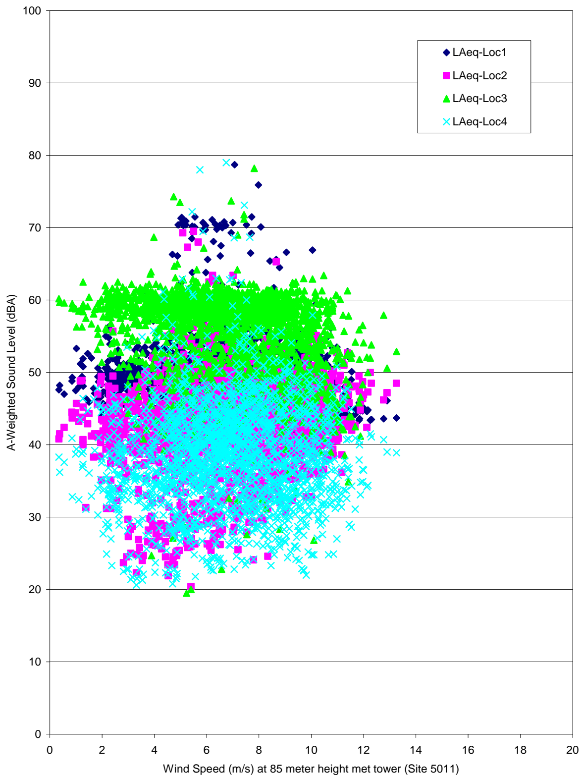
Figure 15. A-Weighted Leq Sound Levels vs. Wind Speed Measured at 10-Minute Intervals at Locations 1 to 4 (23 July – 7 August 2009).
