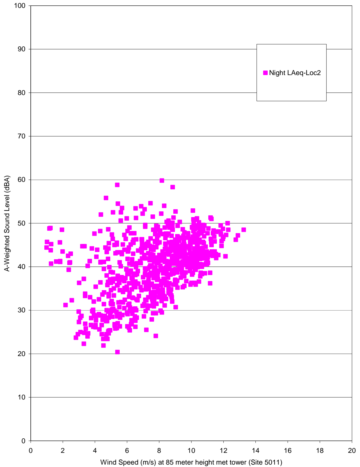
Figure 15f. Nighttime A-Weighted Leq Sound Levels vs. Wind Speed Measured at 10-Minute Intervals at Location 2 (23 July – 7 August 2009).
