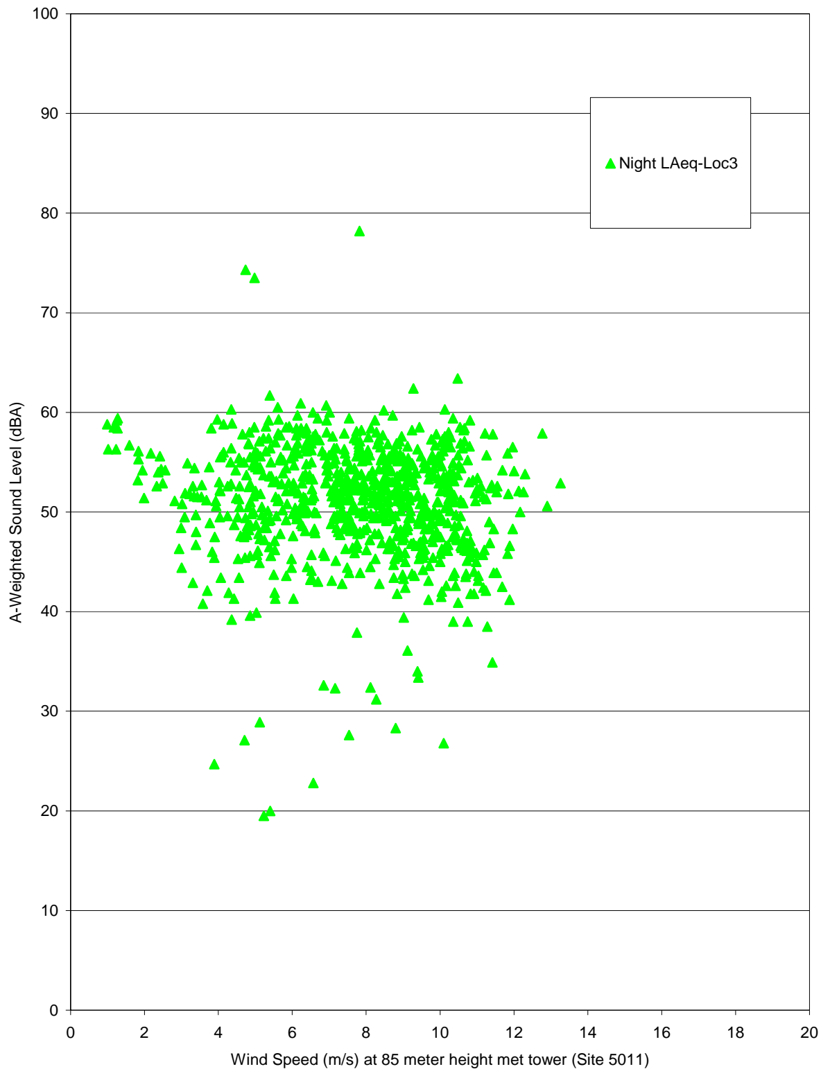
Figure 15g. Nighttime A-Weighted Leq Sound Levels vs. Wind Speed Measured at 10-Minute Intervals at Location 3 (23 July – 7 August 2009).
