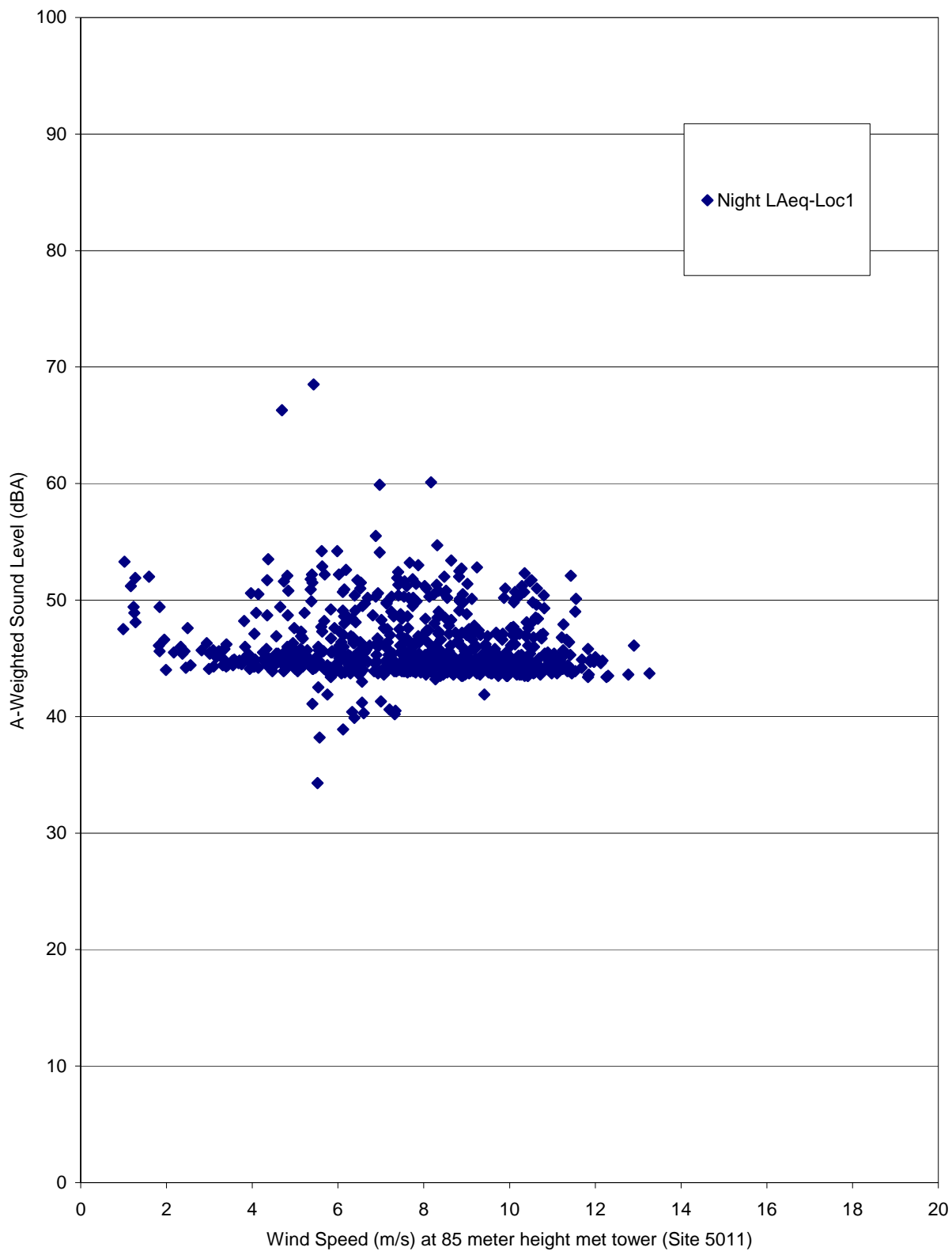
Figure 15e. Nighttime A-Weighted Leq Sound Levels vs. Wind Speed Measured at 10-Minute Intervals at Location 1 (23 July – 7 August 2009).
