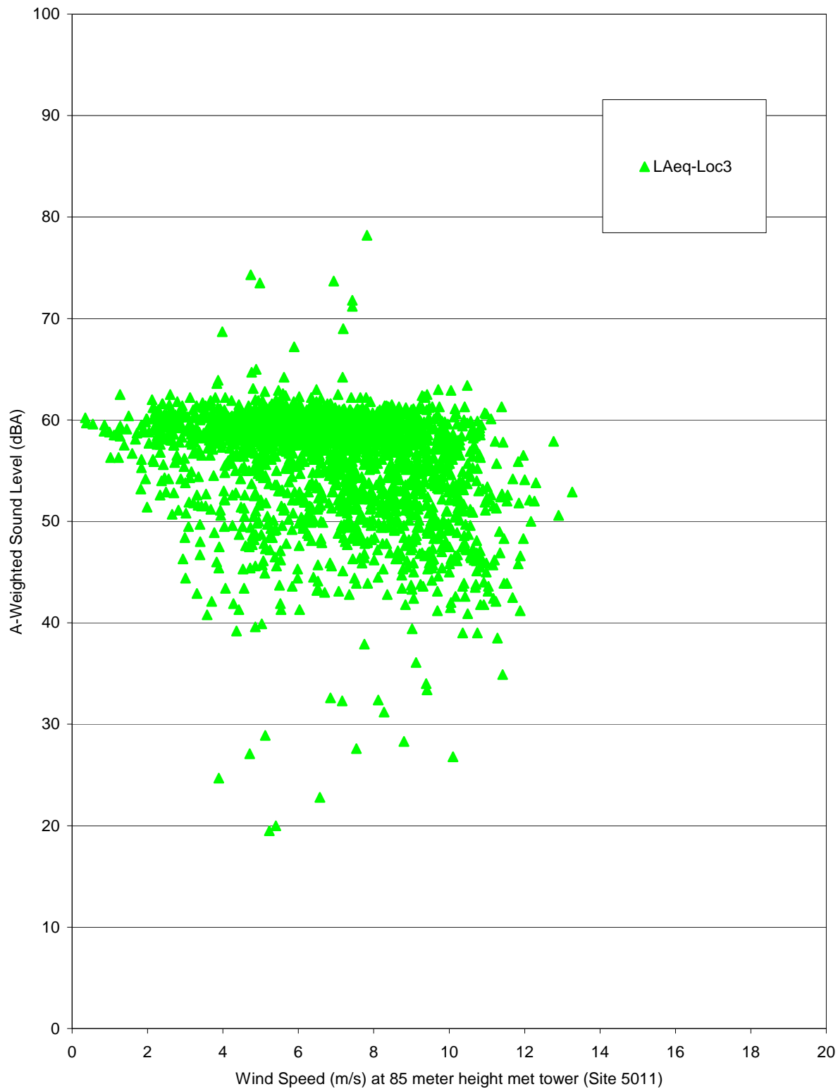
Figure 15c. A-Weighted Leq Sound Levels vs. Wind Speed Measured at 10-Minute Intervals at Location 3 (23 July – 7 August 2009).
